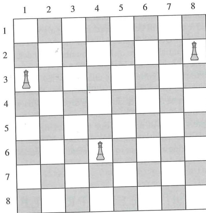
Figure 5.6 The queen in row 6 is being threatened in its left diagonal by the queen in row 3 and in its right diagonal by the queen in row 2.
